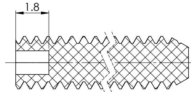
SECTION X-X
